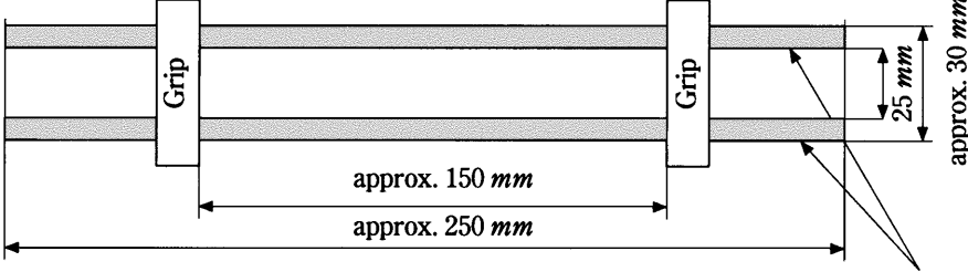
Fig 4.1.2-4 Tensile Test Sample of Roving Cloth
