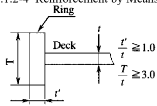
Fig. 5.9.1.2-4 Reinforcement by Means of Ring
