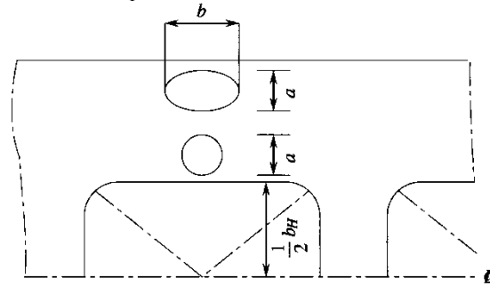
Fig. 4.10.2.3-3 Where Elliptic Hole and Circular Hole are in Same Cross-section
