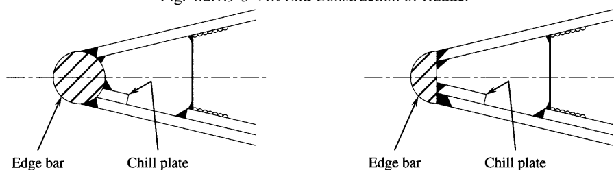
Fig. 4.2.1.9-3 Aft End Construction of Rudder
