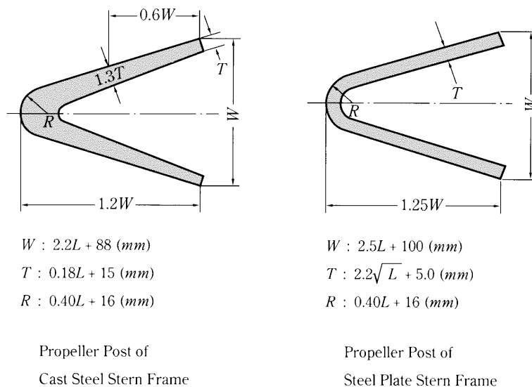
Fig. 4.2.5 Standard Dimensions of Propeller Posts
