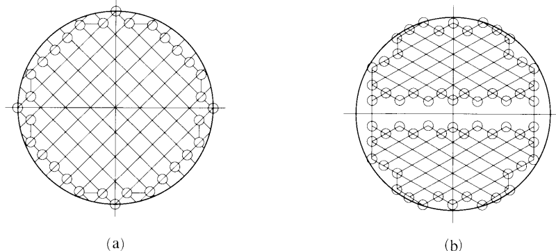
Fig. 7.8.2 Polygon used for Tube Plate Calculation
