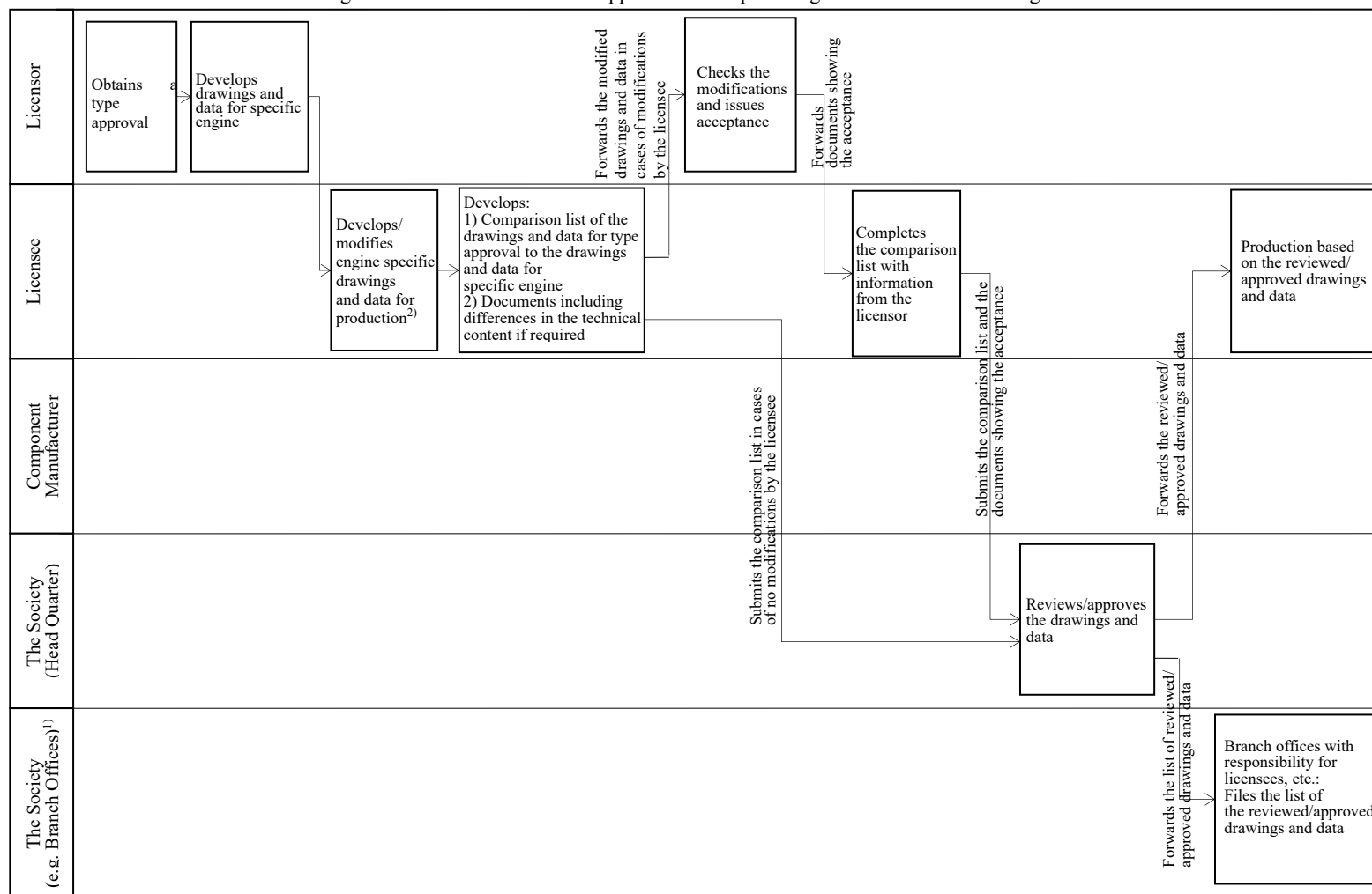
Fig. 7.2.1.4-1 Flow of Approval of Reciprocating Internal Combustion Engines
