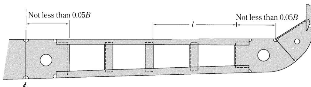
Fig. 4.3.2 Open Floors
