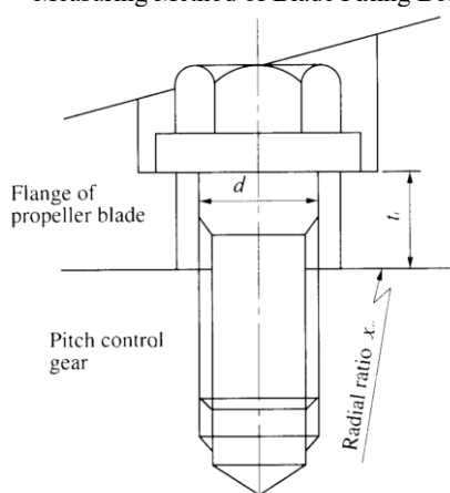
Fig. 7.5.2 Measuring Method of Blade Fixing Bolt Dimensions
