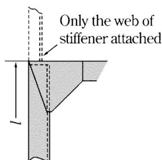
Fig. 4.8.2 Types of End Connection (Connection Type B)
