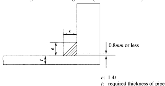
Fig. 7.10.4.3-2 Flange Joint (One-side welded)
