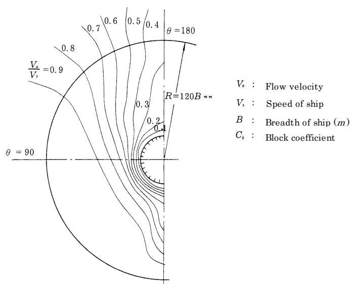
Fig. 7.5.2.1-1 Standard wake distribution for high speed craft
