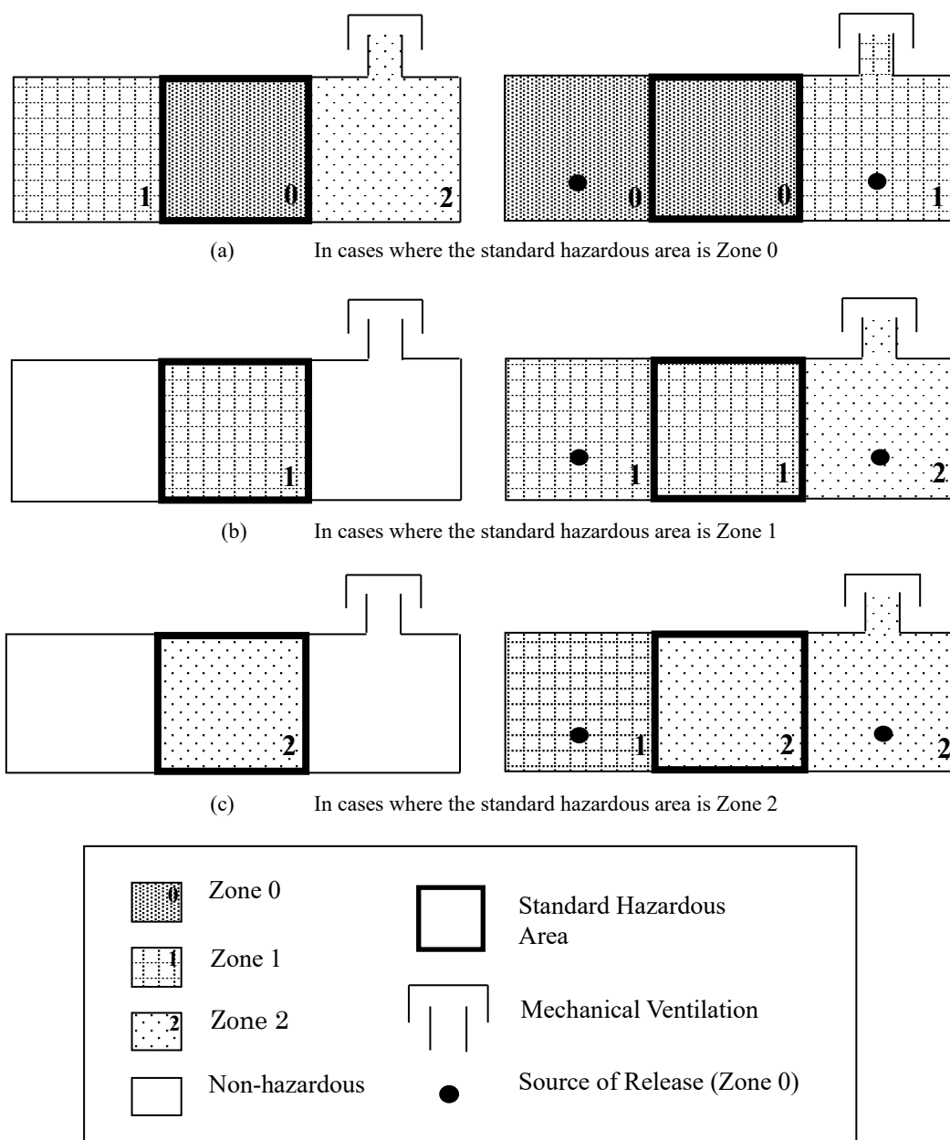
Fig.8.5.9.3-1 Hazardous Areas Adjacent to Standard Hazardous Areas
