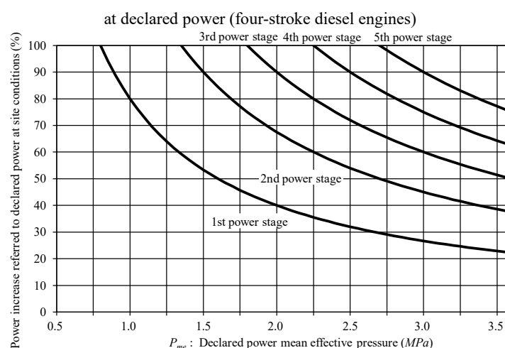
Fig. 7.2.4.1 Reference values for maximum possible sudden power increases as a function of brake mean effective pressure ( P_{me} )
