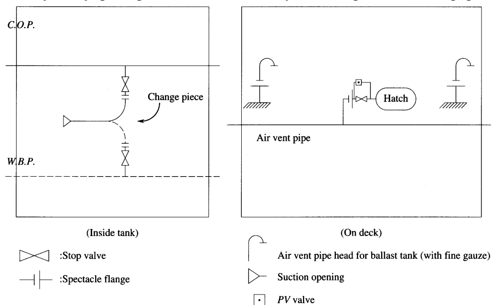
Fig. 7.15.6.4-1 Example of Piping Arrangements for Tanks Alternatively Used as Cargo Oil Tanks and Segregated Ballast Tanks
