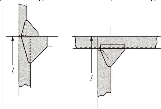
Fig. 4.8.1 Types of End Connection (Connection Type A)
