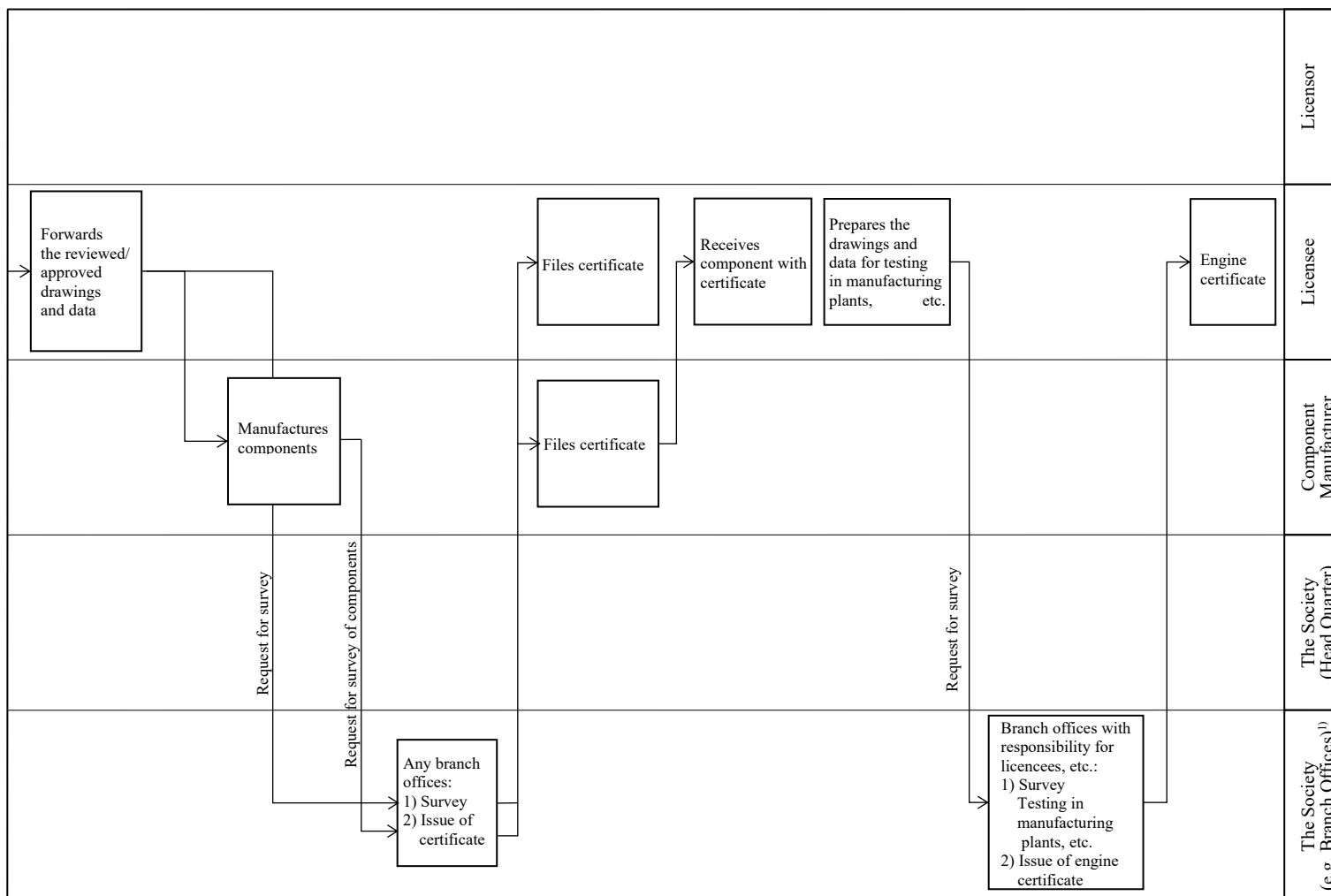
Fig. 7.2.1.4-1 Flow of Approval of Reciprocating Internal Combustion Engines (continued)
