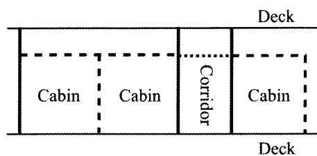
Fig. 7-1-A8 Continuous “B” Class Ceiling(Regulation II-2/9.2.2.2.3)
