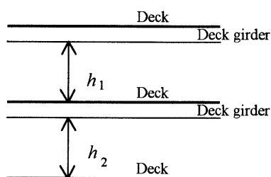
Fig. 7-1-A22 Total Overall Clear Height for Vehicles (Regulation II-2/20.2.2.1)
