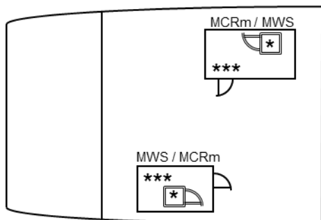
Fig. R13.4.5 Represent typical arrangements of the continuous fire shelters
