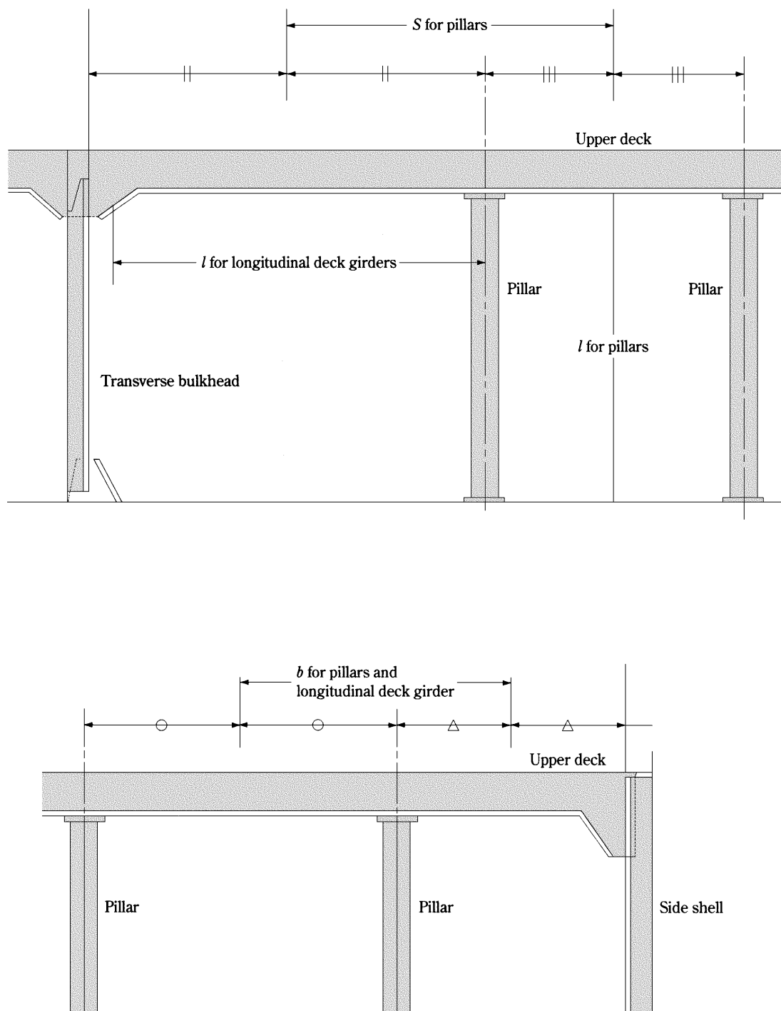
Fig. Q8.1 The Way of Measuring S , b and l for Pillars, Transverse and Longitudinal Girder
