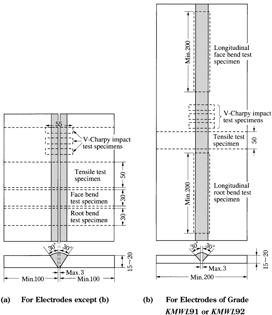
Fig. M6.2 Butt Weld Test Assembly (Unit: mm)
