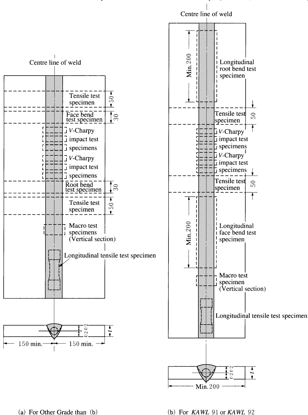
Fig. M6.14 Butt Weld Test Assembly with One-run and Multi-run Technique (Unit: mm , t =Plate thickness)
