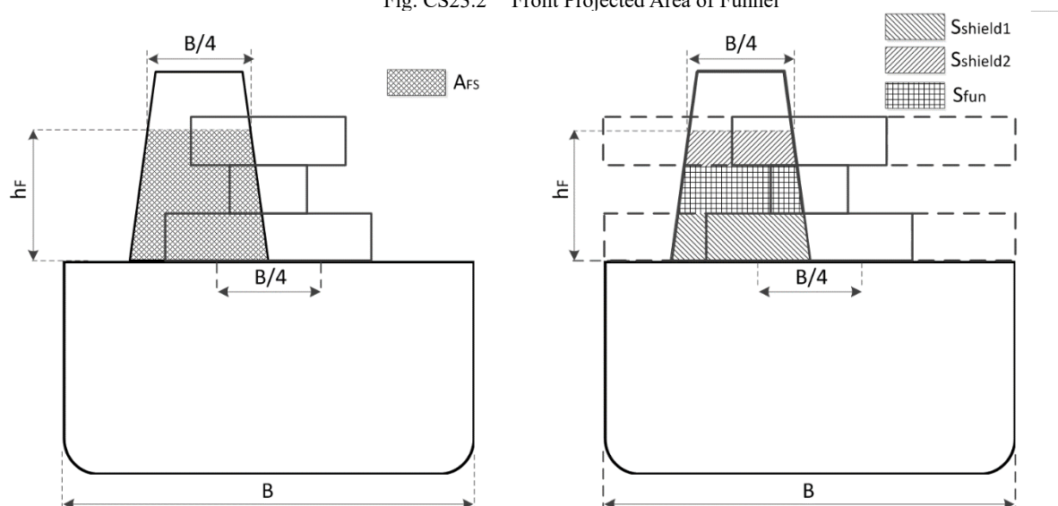
Fig. CS23.2 Front Projected Area of Funnel
