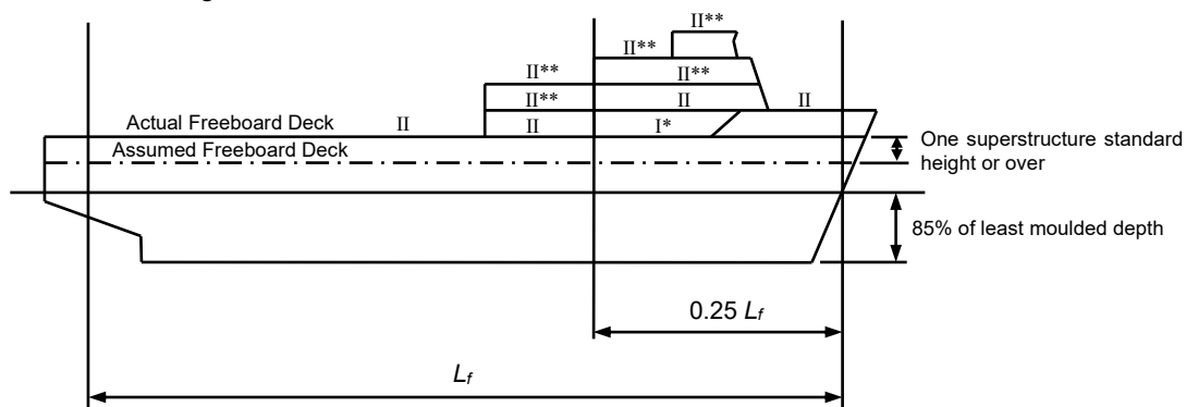
Fig. CS19.2.4-2 Position I and II for an Increased Freeboard
