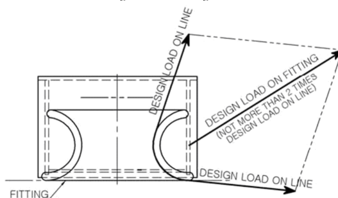
Fig. CS23.7 Design Load
