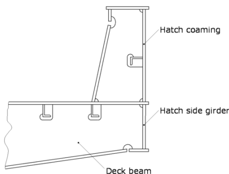
Fig. 1 Example of extension to lower edge of deck beams of longitudinal coaming by fitting a hatch side girder
