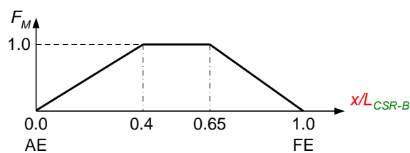
Fig. 3 Distribution Factor F_M
