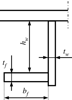
Fig. 5 Net Dimensions of an Angle
