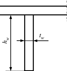
Fig. 3 Net Dimensions of a Flat Bar
