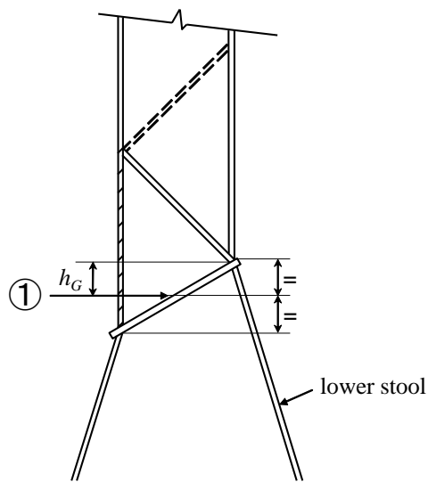
Fig. 15 Asymmetrical Gusset/Shegger Plates
