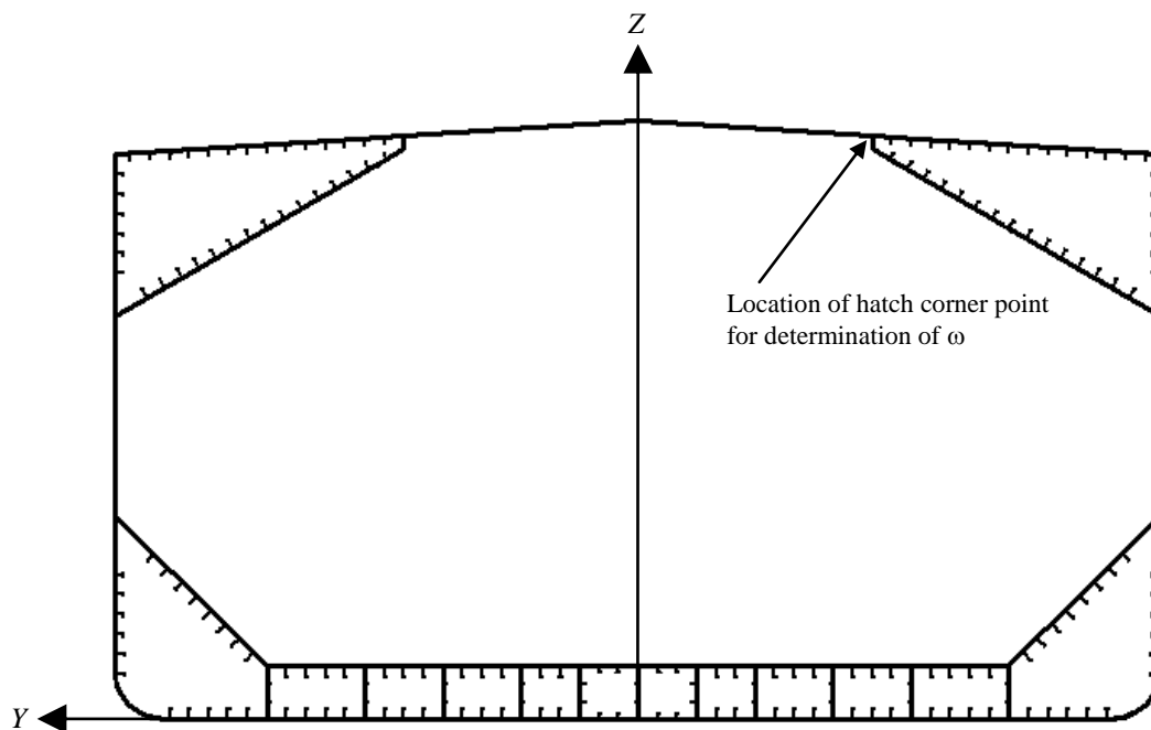
Fig. 1 Cross Section for Determination of I_T and \omega
