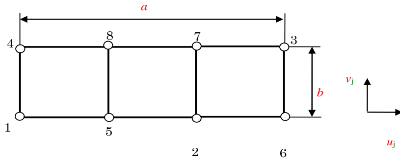
Fig. 2 8-node Buckling Panel (a) Displacement Nodes
