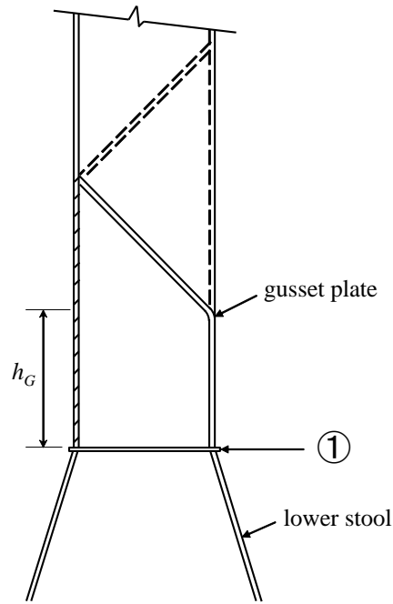
Fig. 14 Asymmetrical Gusset/Shegger Plates
