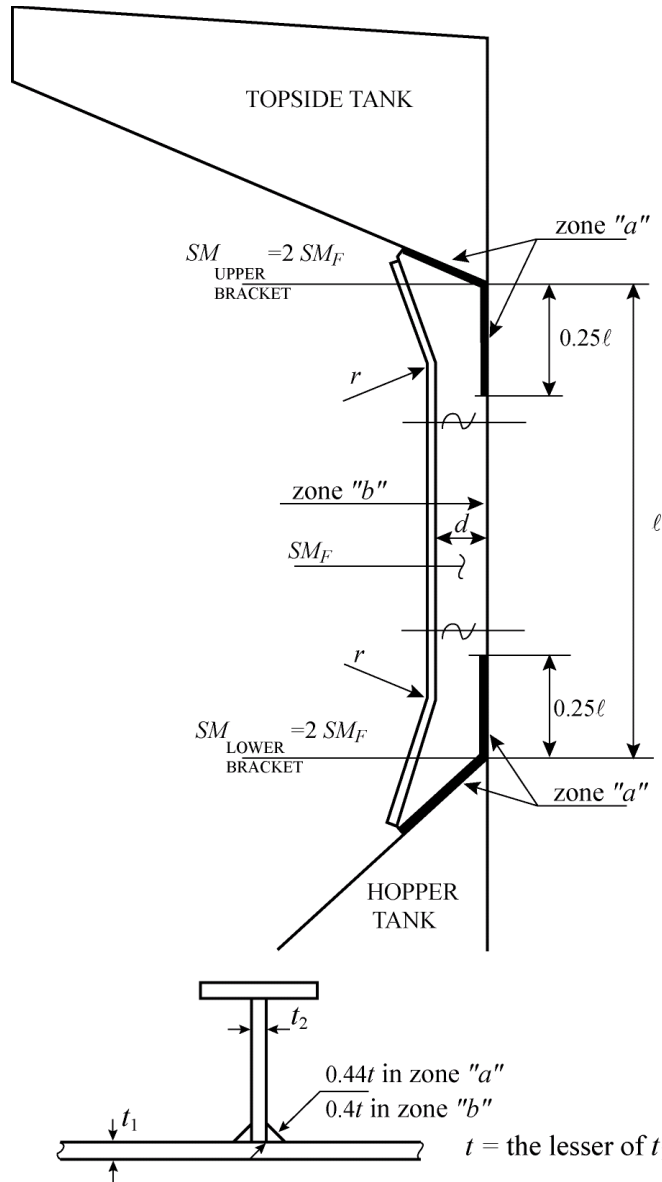
Fig. 20 Dimensions of Lower and Upper Brackets
