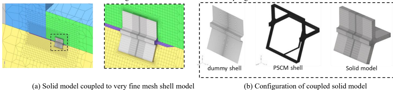
Fig. 9.7.2-1 Shell-Solid Model Coupling Procedure
