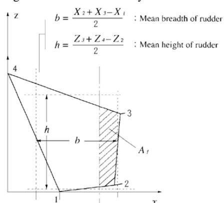
Fig. 13.2.2-1 Coordinate System of Rudders
