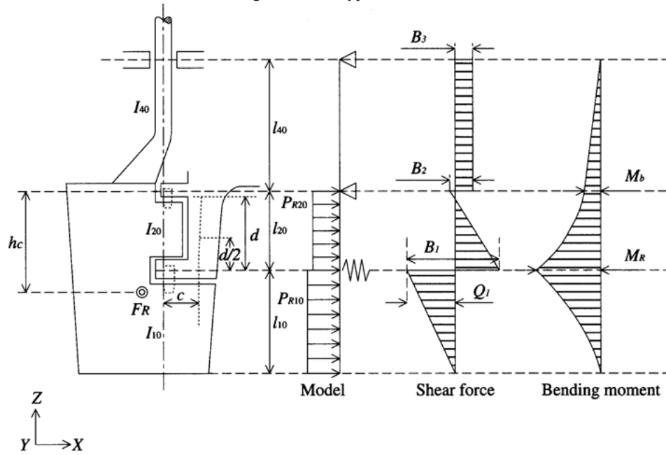
Fig. C13.2.4-5 Type E Rudder
