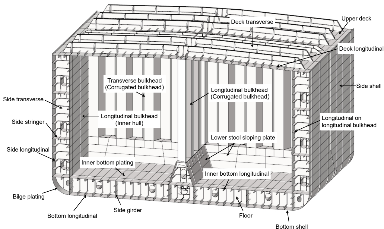
Fig. 1.4.5-9 Chemical Tanker
