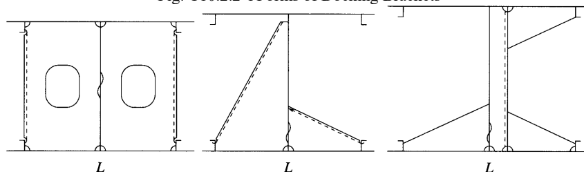
Fig. C10.2.2-1 Forms of Docking Brackets
