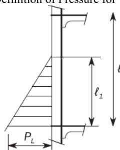
Fig. An6 Definition of Pressure for Vertical Stiffeners
