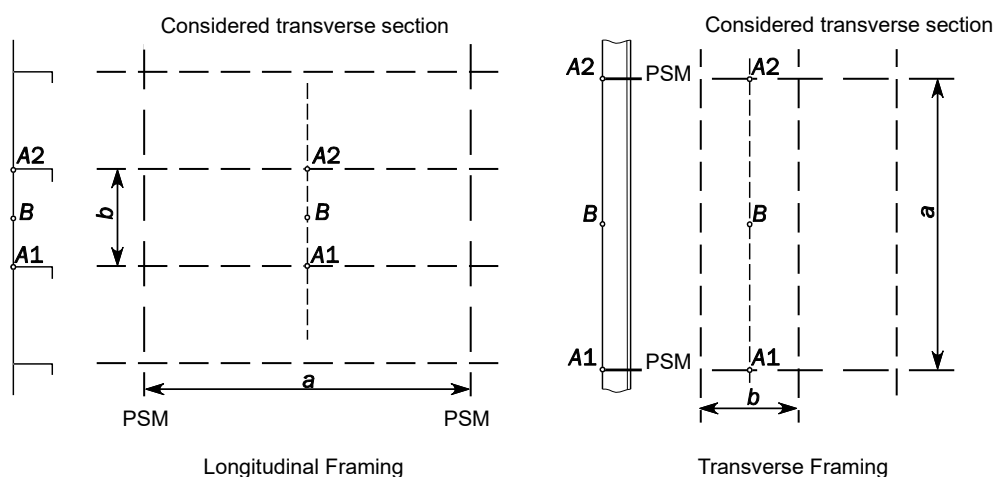
Fig. An5 LCP for Plate Buckling Assessment
