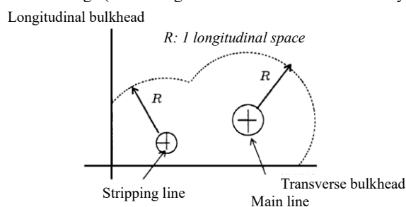
Fig. 3.3.4-2 Thickness Increase Range (With Longitudinal Bulkhead in the Vicinity of the Suction Bellmouth)
