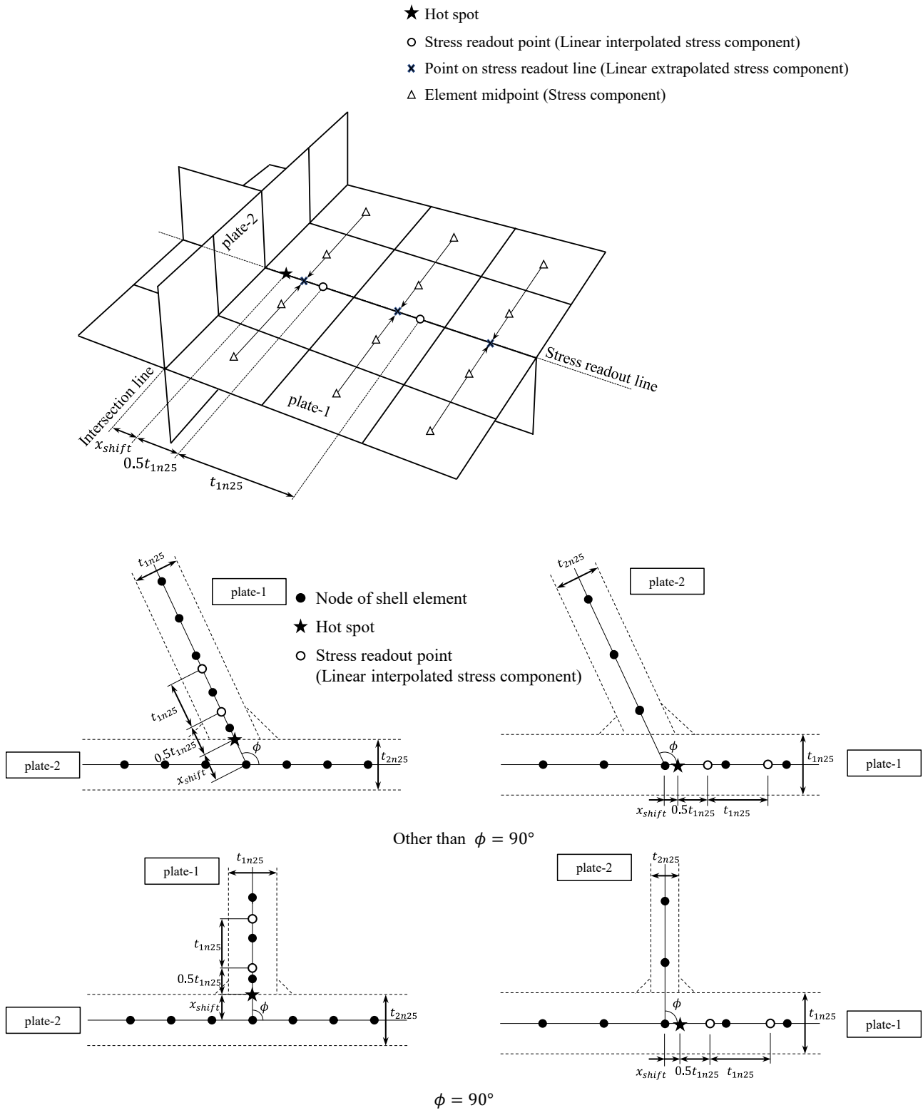
Fig. 9.4.5-2 Location and Readout Method for Type “a1-0” Hot Spot Stress
