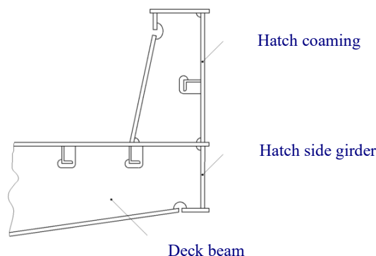
Fig. 14.6.9-2 Example for the Extension of Coaming Plates
