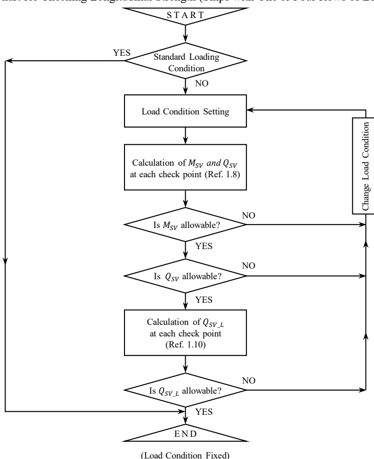
Fig. 6 Flow Chart for Checking Longitudinal Strength (Ships with One or Four Rows of Longitudinal Bulkheads)
