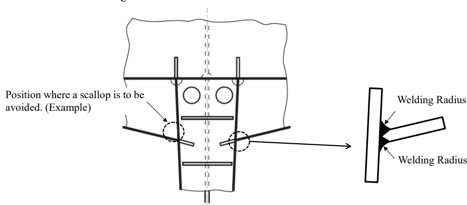
Fig. 11.5.1-4 Connection of Rudder Horn and Hull
