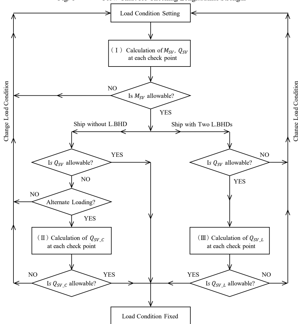
Fig. 1 Flow Chart for Checking Longitudinal Strength
