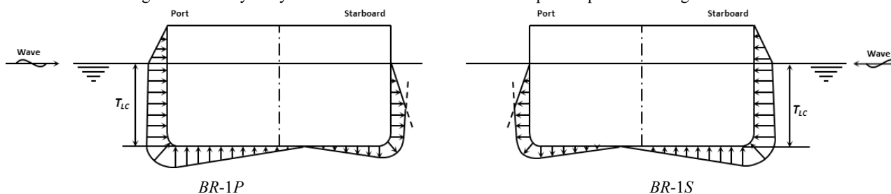
Fig. 4.7.2-3 Hydrodynamic Pressure Distribution Amidships in Equivalent Design Wave BR
