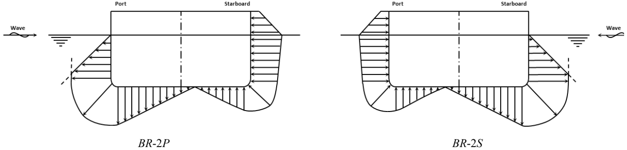
Fig. 4.6.2-4 Hydrodynamic Pressure Distribution Amidships in Equivalent Design Wave BR
