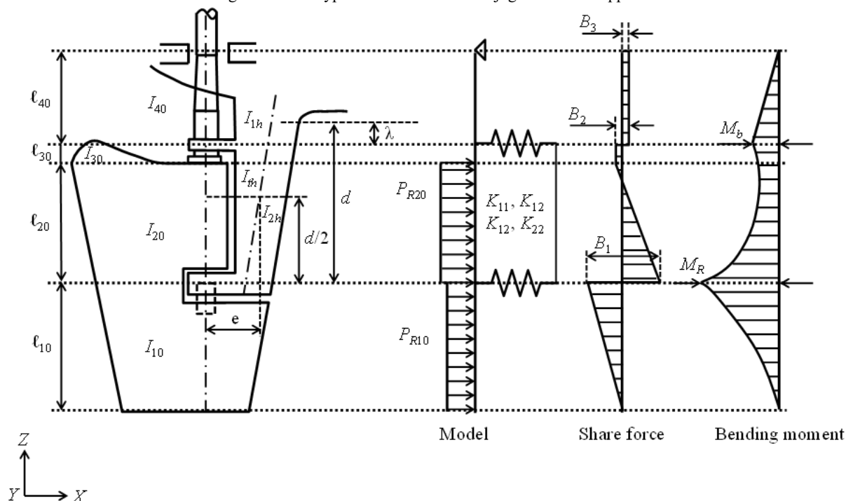
Fig. C13.2.4-8 Type D Rudder with 2-conjugate Elastic Supports
