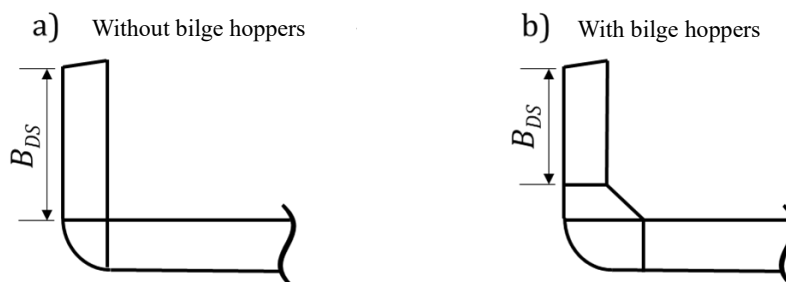
Fig. 7.3.1-4 Breadth of Double Side
