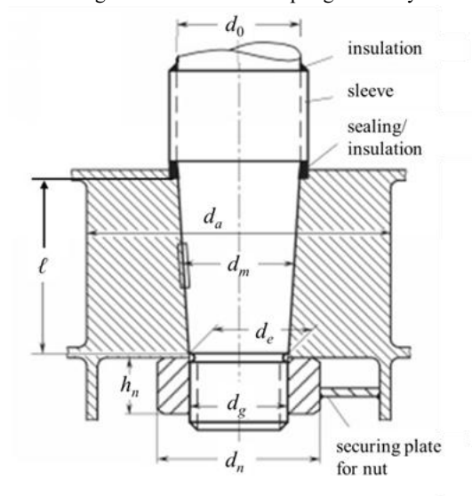
Fig. 13.2.8-2 Cone Coupling with Key
