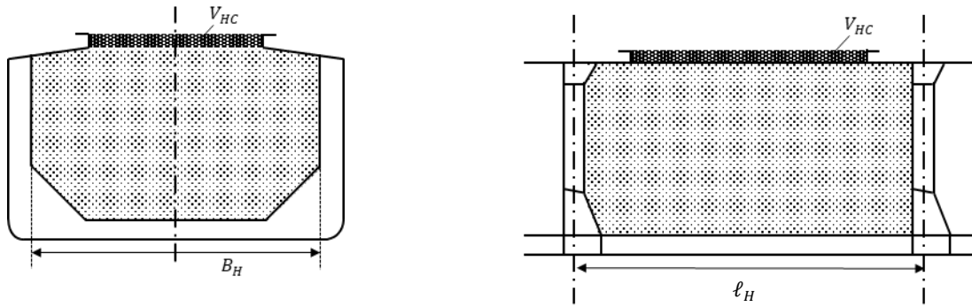
Fig. 4.4.2-2 Cargo Hold Loaded with Dry Bulk Cargo
