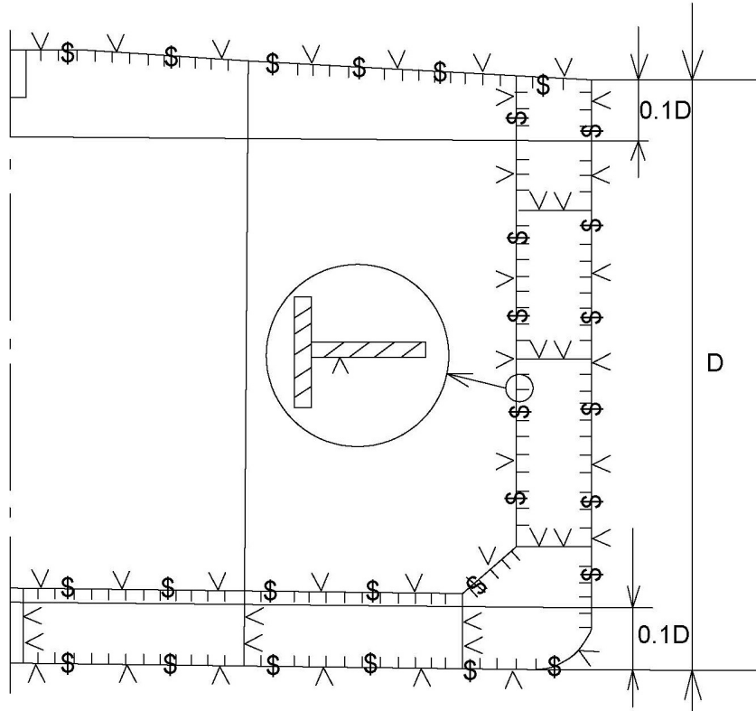
Figure 5 - Transverse section
