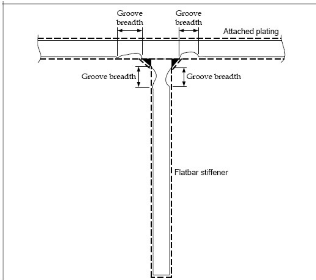
Figure 3 - Grooving corrosion
